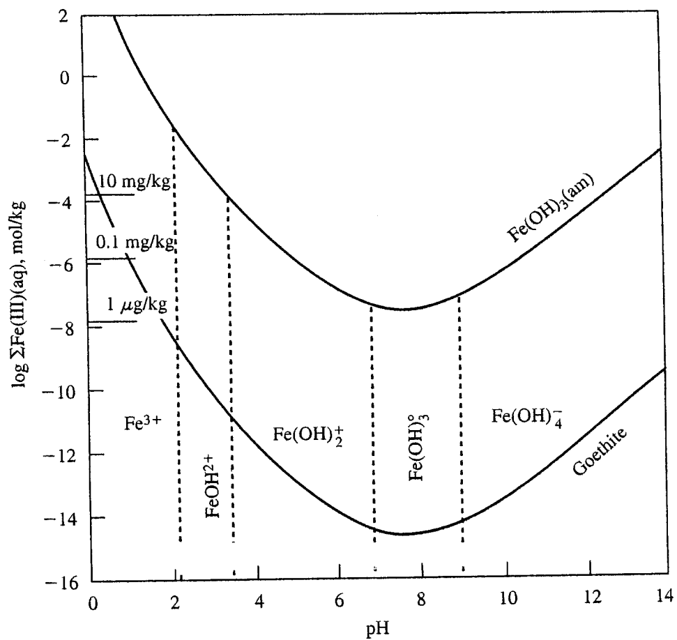
Figure 13. Solubility of amorphous \text{Fe(OH)}_3 , \text{pK}_{\text{sp}} = 37.1 (top curve), and goethite [ \alpha - \text{FeOOH} ], \text{pK}_{\text{sp}} = 44.2 (bottom curve) as a function of pH at 25° C. Also shown are fields of dominance of \text{Fe}^{3+} ion and \text{Fe}^{3+} -OH complexes. After Langmuir, 1997a.
