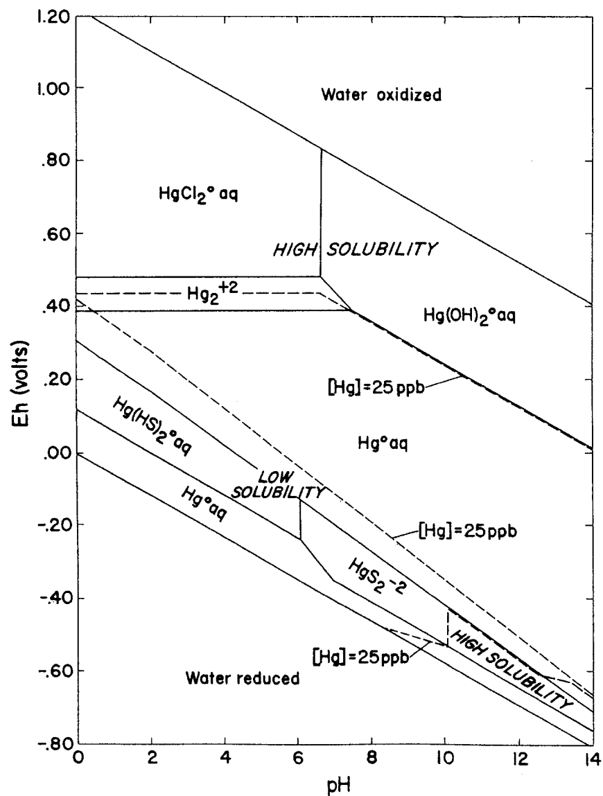
Figure 28. Eh-pH diagram for the system \text{Hg-O}_2\text{-Cl-S-H}_2\text{O} , assuming that \Sigma\text{Hg} = 10^{-6.9} mol/kg, \Sigma\text{Cl} = 10^{-3} mol/kg, and \Sigma\text{S} = 10^{-3} mol/kg. Diagram shows the importance of Hg-Cl complexing. After Bodek et al., 1988.
