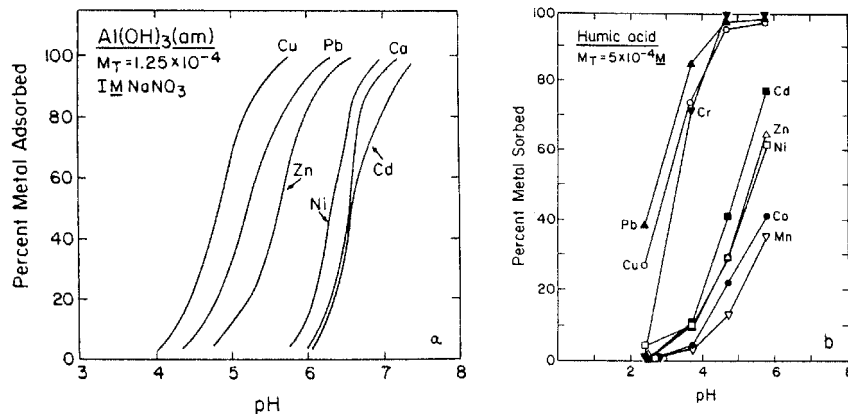
Figure 8. Percent metal adsorbed: (a) by \text{Al}(\text{OH})_3(\text{am}) at total metal concentrations of 1.25 \times 10^{-4} M in 1 M \text{NaNO}_3 solutions, and (b) by humic acid at total metal concentrations of 5 \times 10^{-4} M. From Sposito, 1984.
