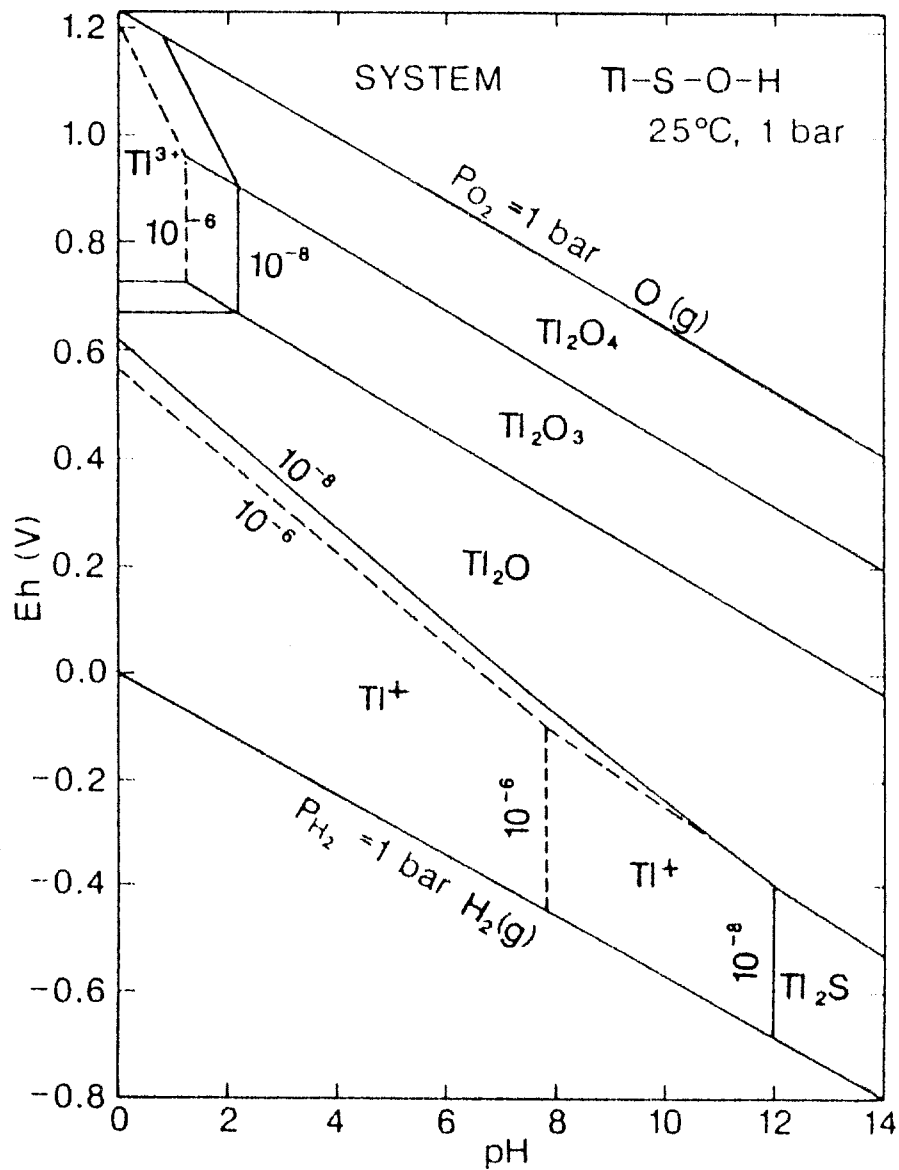
Figure 29. Eh-pH diagram for the system \text{Tl-O}_2\text{-S-H}_2\text{O} , assuming that \Sigma\text{Tl} = 10^{-8} and 10^{-6} mol/kg and \Sigma\text{S} = 10^{-3} mol/kg. The diagram shows the insolubility of the higher-valent Tl oxides under oxidizing conditions. After Brookins, 1988.
