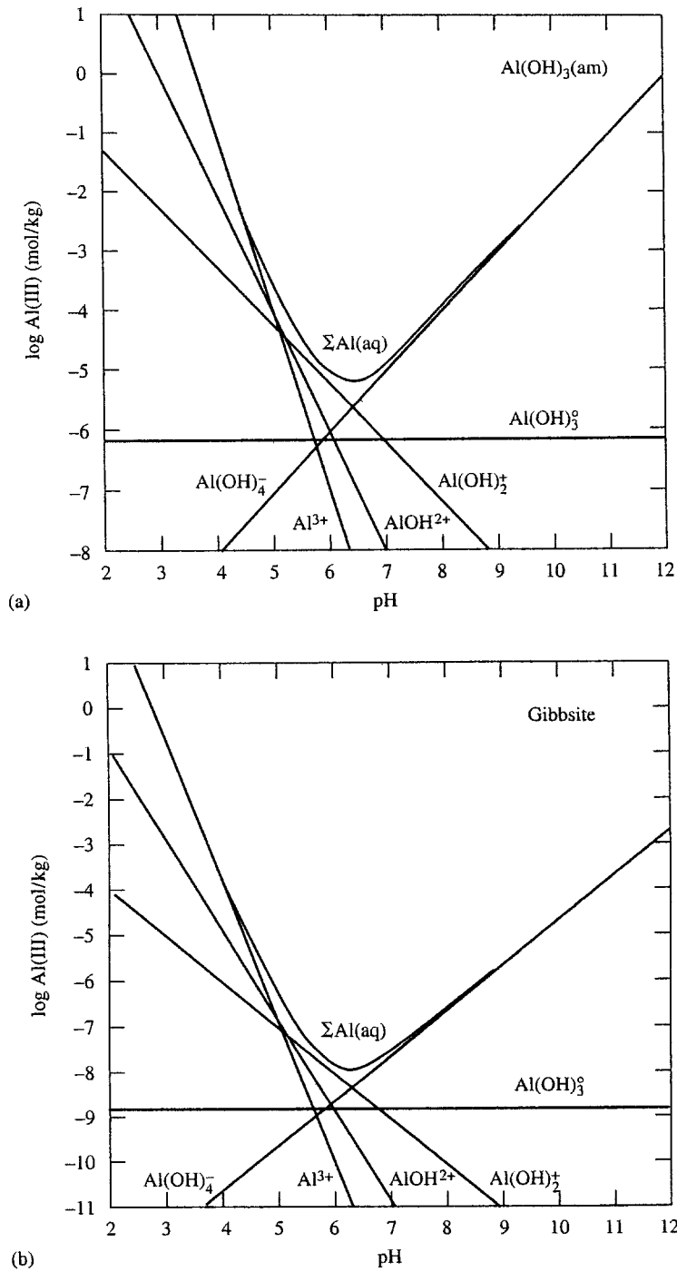
Figure 17. Solubility of (a) amorphous \text{Al(OH)}_3 , K_{\text{sp}} = 10^{-31.2} and (b) gibbsite ( \text{Al[OH]}_3 ), K_{\text{sp}} = 10^{-33.9} , as a function of pH at 25°C. Also shown are lines indicating the solubility contributions of \text{Al}^{3+} and individual Al-hydroxy complexes. From Langmuir, 1997a.
