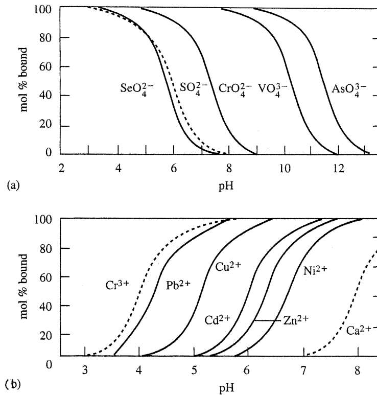
Figure 7. Adsorption of various metal cations and oxyanions, each at 5 \times 10^{-7} \text{ M} , by ferrihydrite ( \Sigma\text{Fe[III]} = 10^{-3} \text{ M} ) as a function of pH at an ionic strength of 0.1 \text{ mol/kg} . There are 2 \times 10^{-4} \text{ M} of reactive sites on the oxyhydroxide. The dashed curves are calculated. After Stumm, 1992.
