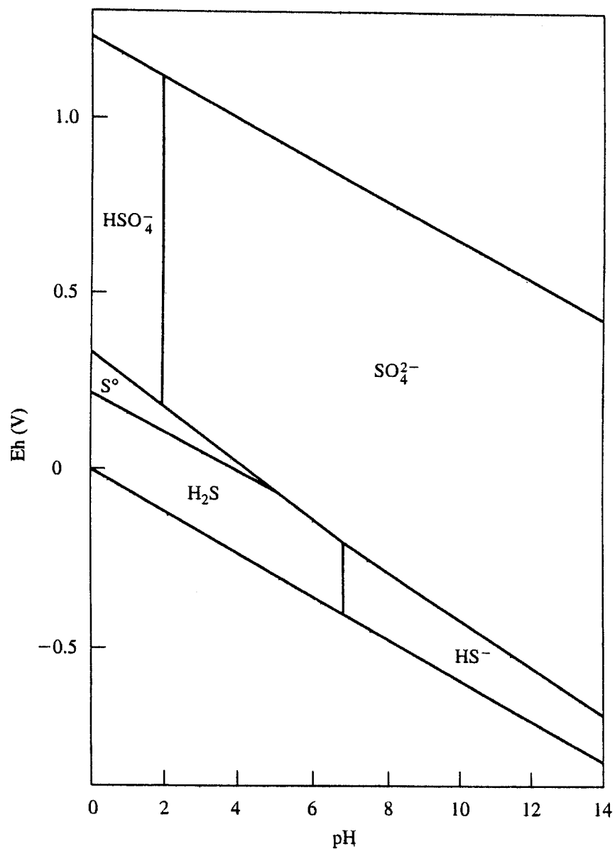
Figure 15. Eh-pH diagram for the system S-O 2 -H 2 O at 25° C, showing the fields of predominance of the aqueous species and of elemental sulfur (S ° ) for \Sigma S(aq) = 10^{-3} mol/kg at aqueous/S ° boundaries. After Langmuir, 1997a.
