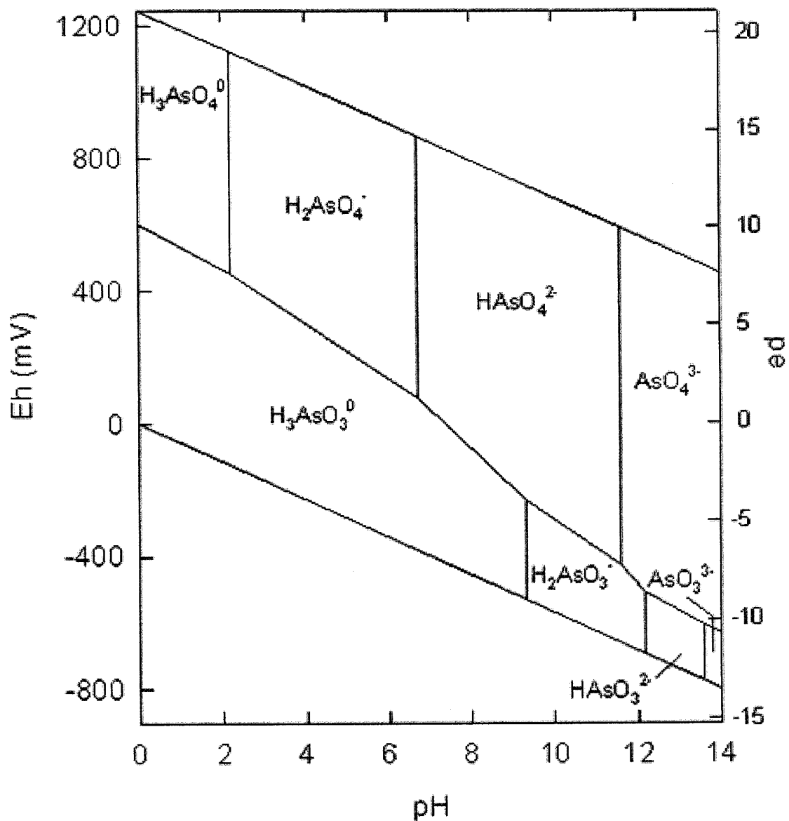
Figure 30. Eh-pH diagram for the system \text{As-O}_2\text{-H}_2\text{O} showing the relative stabilities of arsenate (arsenic acid, As[V]) and arsenite (arsenious acid, As[III]) species under oxidizing and reducing conditions.
