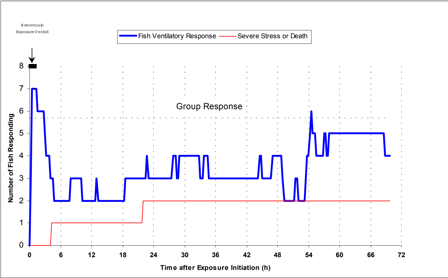
Figure 3-1. Fish ventilatory responses to brevetoxin. An individual fish response is due to a significant change in at least one of the ventilatory parameters (ventilatory rate, ventilatory depth, or cough rate). In this test, a fish group response (six or more fish responding simultaneously) occurred within 30 minutes of the initiation of brevetoxin exposure as a result of increased cough and ventilation rates.
