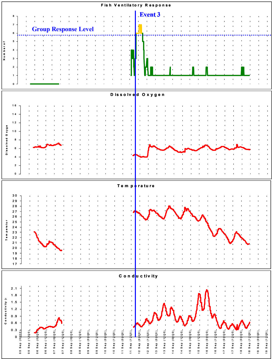
Figure 3-10. Fish ventilatory responses and water quality data during field deployment, September 5 to 18, 2000. a. Ventilatory responses with dissolved oxygen, temperature, and conductivity data. The gap in the data was caused by a software problem. The event was associated with increased cough rate. Although there was a substantial temperature rise, temperature was stable for six hours prior to the event. No definitive cause could be determined, although 2-(2-butoxyethanol)ethanol acetate was detected in water samples.
