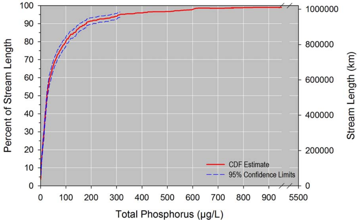
Fig 280-2: Cumulative distribution function for total phosphorus in wadeable streams in the United States
