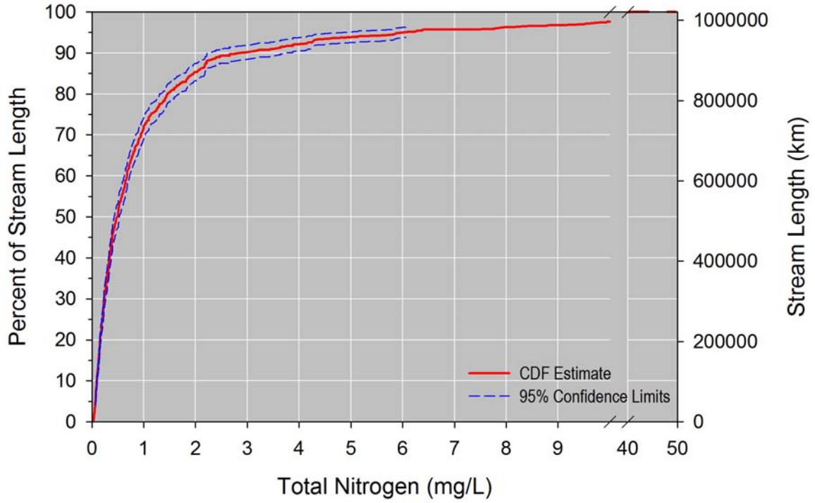
Fig 280-1: Cumulative distribution function for total nitrogen in wadeable streams in the United States
