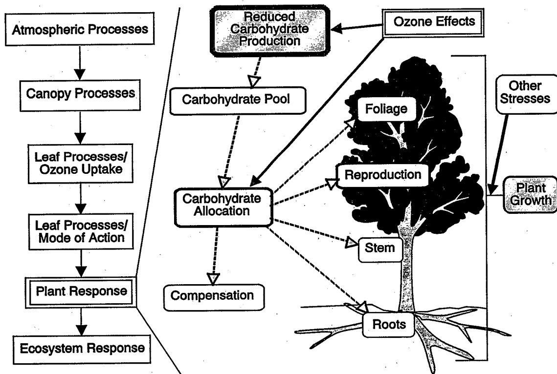
Figure 5-6. Effect of ozone (O 3 ) on plant function and growth. Reduction in carbohydrate allocation affects the pool of carbohydrates available for growth. Changes in relative growth rate of various organs as a function of O 3 exposure suggest that allocation patterns of carbohydrate are affected. Solid black arrows denote where O 3 absorption affects the allocation processes of the plant; dotted arrows show the cascade to plant growth. Boxes with dark borders indicate site of impact. The box with a double border, at left, indicates the location of response.
