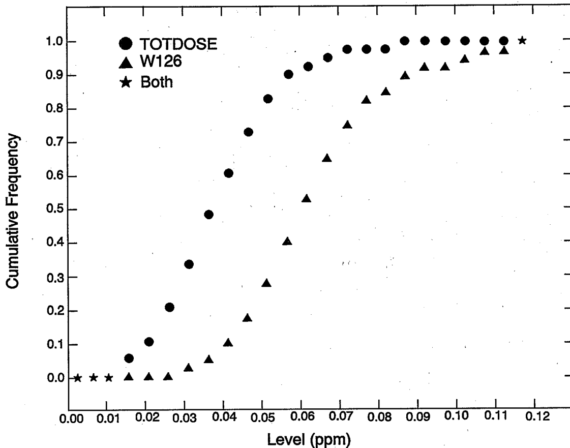
Figure 5-21. A comparison between the resulting cumulative frequencies for the exposure parameters, sum of all hourly average concentrations (SUM00) and the sigmoidally weighted integrated exposure index, W126. The ozone data were collected in 1981 at a site located in the Mark Twain National Forest, MO, EPA AIRS site number 291230001 (Lefohn et al., 1989).
