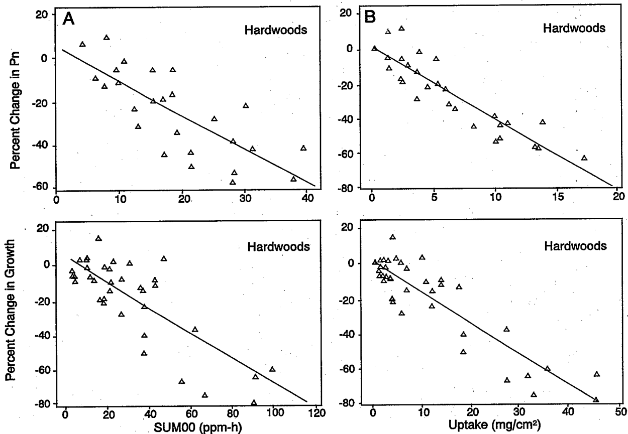
Figure 5-17. Percent reduction in net photosynthesis (Pn) and biomass growth of hardwood species in relation to (A) total exposure (SUM00) and (B) estimated total ozone uptake (Reich, 1987).
