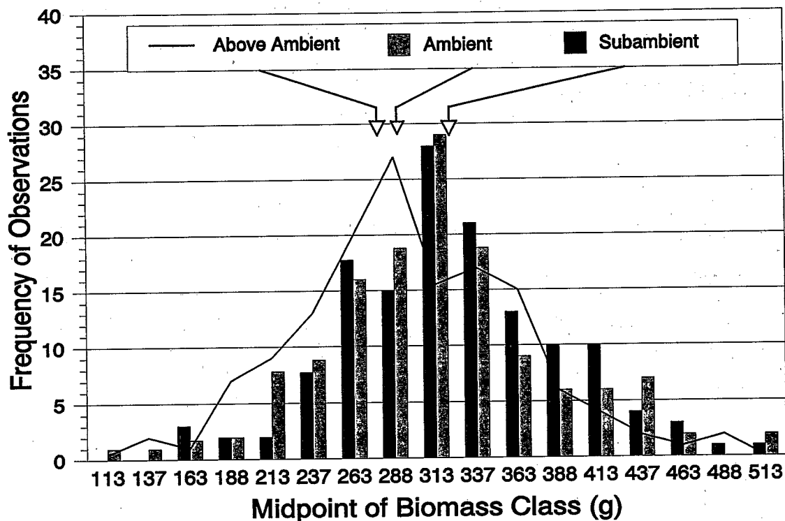
Figure 5-8. Frequency distribution showing the variability in ozone ( O_3 ) response (midpoint of whole-plant biomass) within one half-sib family of loblolly pine ( P. taeda L.) exposed to increasing levels of O_3 under chronic-level field conditions over several growing seasons (Adams et al., 1988). The arrows show the mean response for each of the three O_3 treatments (subambient, ambient, and above-ambient O_3 ). The specifics of the experimental design are reported by Adams et al. (1988). This figure was developed by Taylor (1994).
