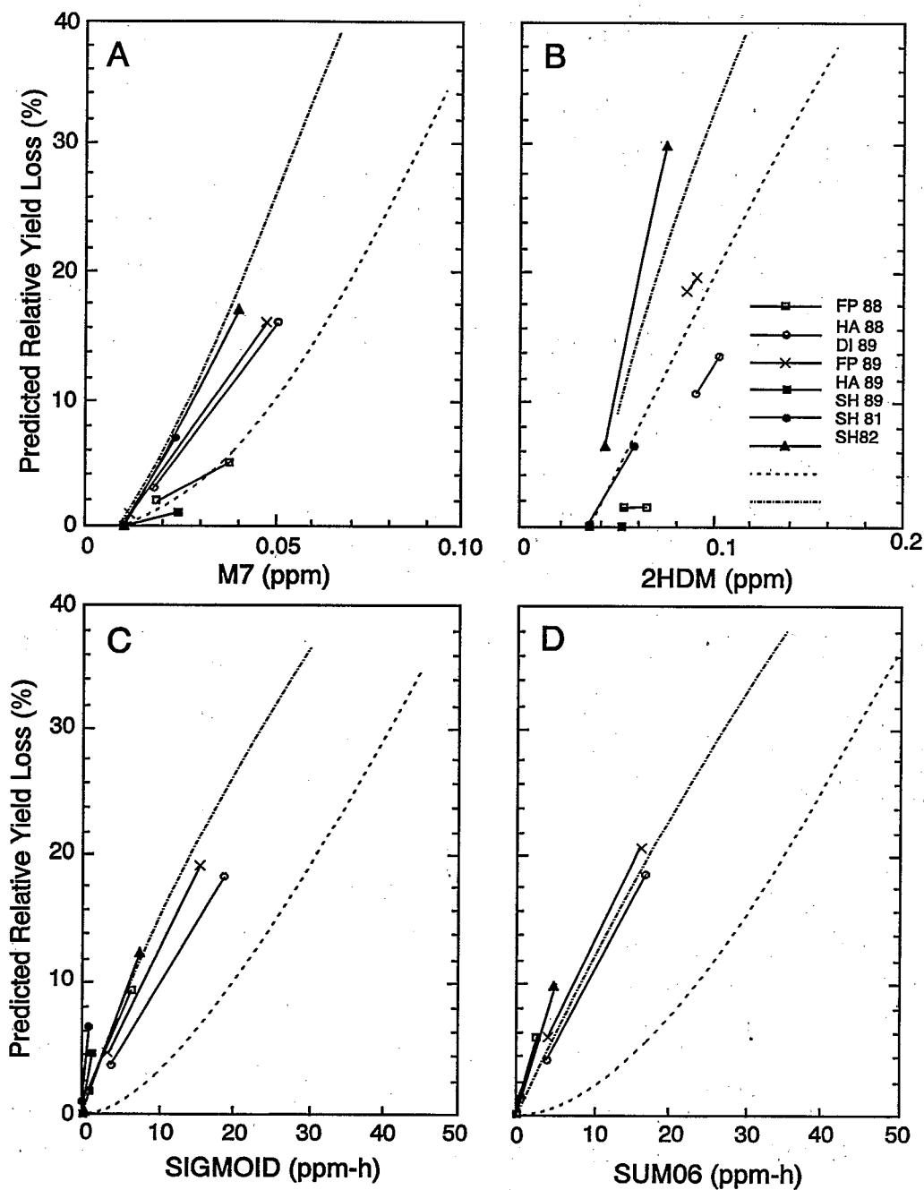
Figure 5-11. Predicted relative yield losses (lint weight) for Acala SJ-2 cotton for four sites and multiple years (1981, 1982, 1988, and 1989) relative to 0.01 ppm for M7, 0.035 ppm for 2HDM, 0 ppm-h for SIGMOID, and 0 ppm-h for SUM06, which correspond to typical levels in the charcoal-filtered chambers. Predicted losses are based on M7 (A), 2HDM (B), SIGMOID (C), and SUM06 (D) exposure indices. Abbreviations: DI = Dinuba, FP = Five Point, HA = Hanford, and SH = Shafter (Olszyk et al., 1993).
