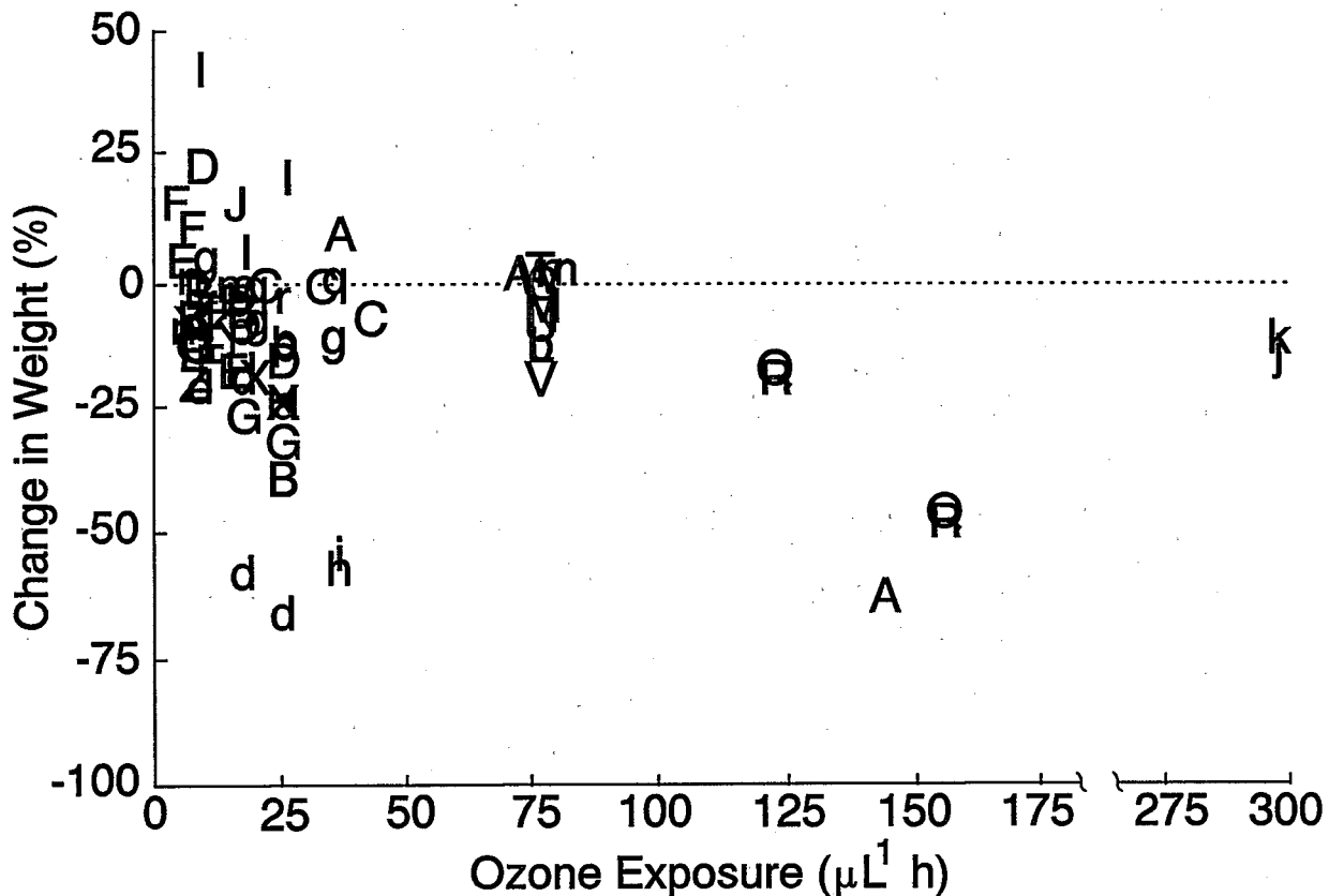
Figure 5-19. Percent reduction in biomass growth of tree seedlings in relation to total exposure (Pye, 1988).
