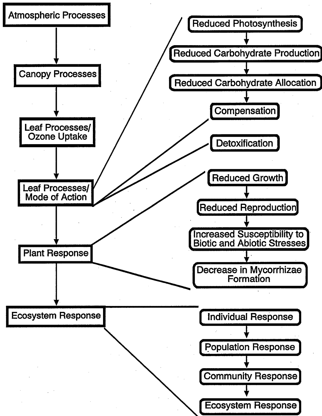
Figure 5-1. Leaf absorption and possible functional changes that may occur within the plant. Ecosystem response begins at the level of the individual and is propagated to the more complex level of organization.
