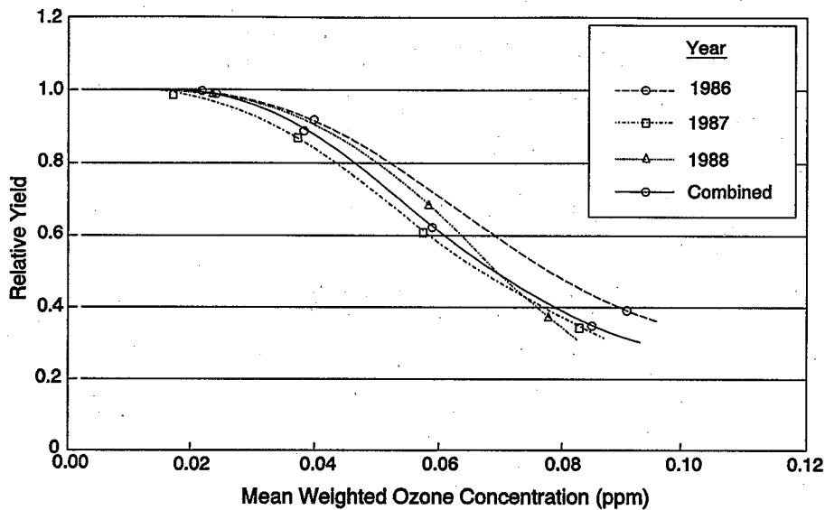
Figure 5-13. Weibull exposure-response curves for the relative effect of ozone on grain yield of spring wheat for 3 years, individually and combined (Fuhrer et al., 1989).
