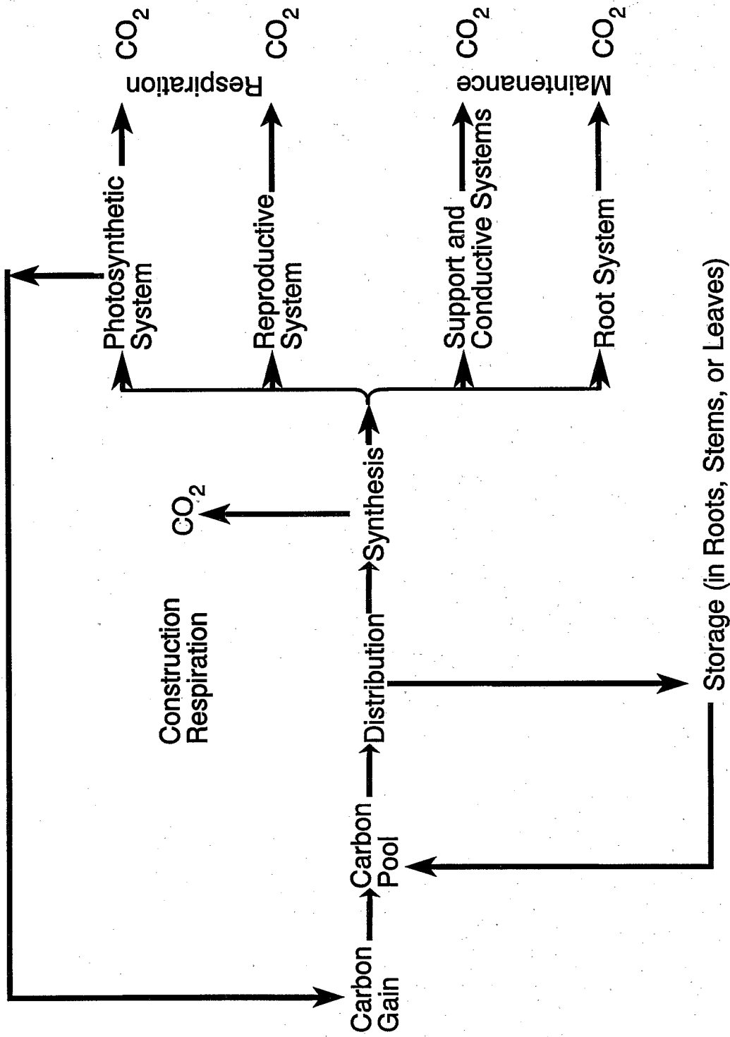
Figure 5-34. Carbon uptake through photosynthesis is made available to a general pool of carbohydrates used in construction and maintenance of various tissues. Carbohydrates may be shifted from one category to another, depending on environmental conditions.
