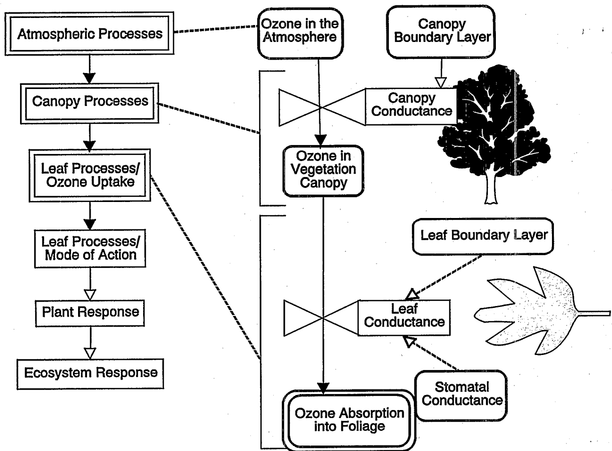
Figure 5-2. Uptake of ozone ( O_3 ) from the atmosphere. Ozone is moved from the atmosphere above the canopy boundary layer into the canopy primarily by turbulent flow of air. Canopy conductance, controlled by the complexity of the canopy architecture and the wide distribution within the canopy, is a measure of the ease with which gases move into the canopy. Within the canopy, O_3 can be adsorbed by surfaces as well as being absorbed into the foliage. Foliage absorption is controlled by two conductances, leaf boundary layer and stomatal, which together determine leaf conductance. The solid black arrows denote O_3 flow; dotted arrows indicate processes affecting uptake or response to O_3 . Boxes at the left with double borders are those processes described in the figure. The rounded box with a double border is the end of pathway on this figure.
