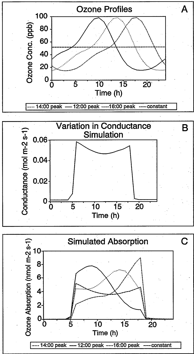
Figure 5-4. Simulation of the effects of diurnal variation in stomatal aperture and in ozone ( O_3 ) concentration on O_3 uptake: (A) diurnal O_3 concentrations, (B) simulated conductance, and (C) O_3 uptake.
