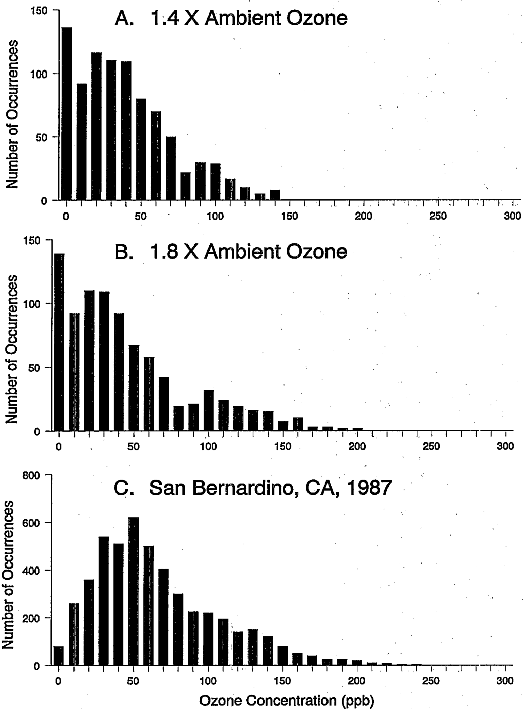
Figure 5-9. Distribution pattern showing the number of ozone concentrations within specified ranges for the 1983 winter wheat proportional-addition experiment for the (A) 1.4 × ambient air and (B) 1.8 × ambient air treatments and for (C) San Bernardino, CA, in 1987.
