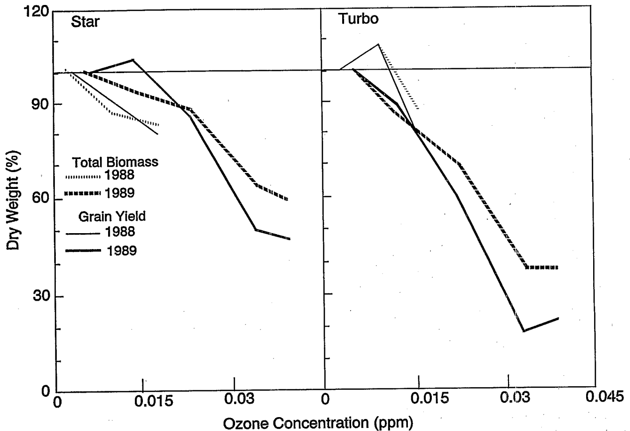
Figure 5-12. Relative effect of ozone on growth and yield of spring wheat cultivars (var. Star and Turbo) from two growing seasons (Adaros et al., 1991a).
