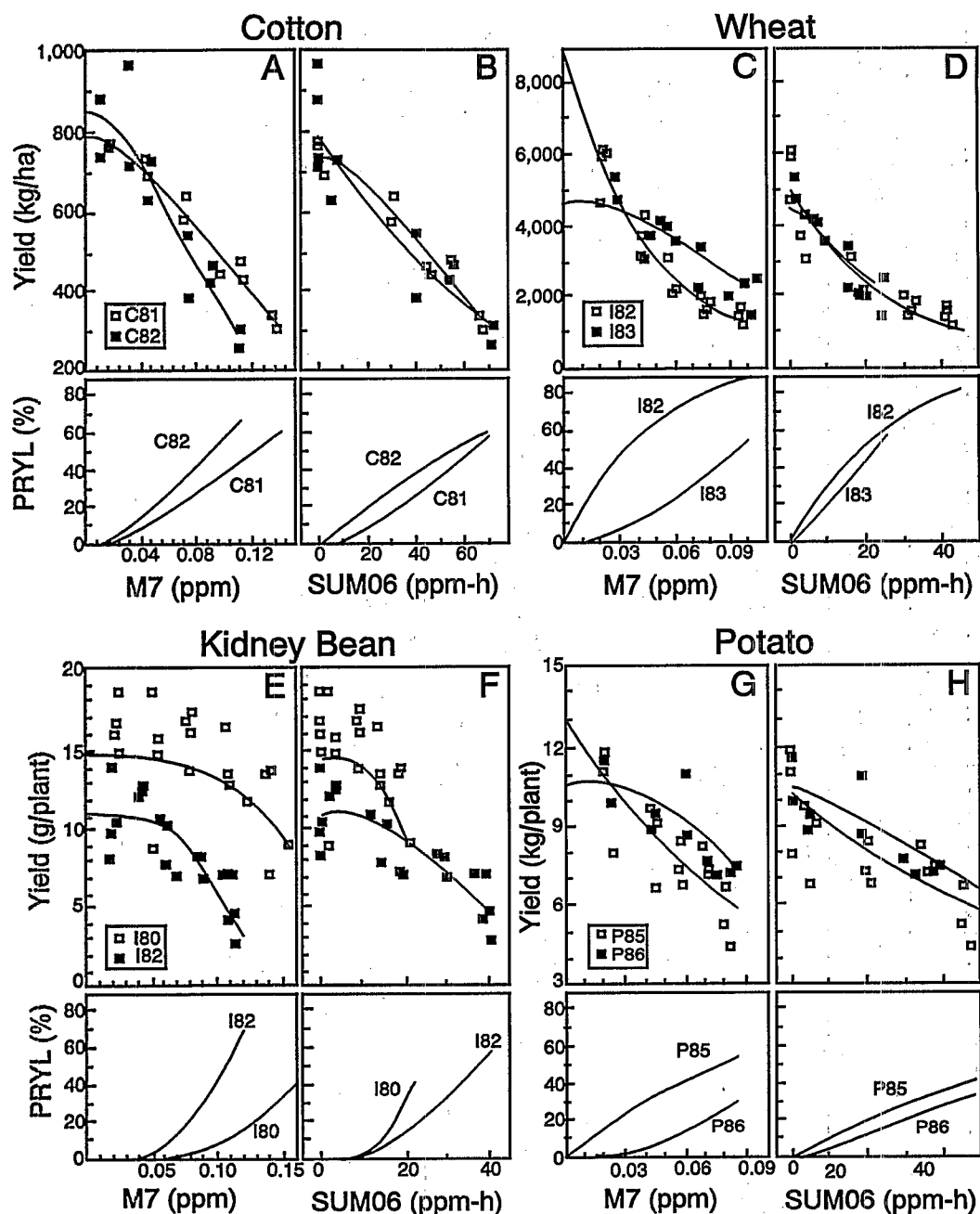
Figure 5-10. Comparison of the Weibull exposure-response functions and its predicted relative yield loss (PRYL) curves (relative to 0 ozone) using M7 and daytime SUM06 for replicate years of National Crop Loss Assessment Network Program's data for (A) and (B) cotton (var. Acala SJ-2), (C) and (D) wheat (var. Vona), (E) and (F) kidney bean (var. California light red), and (G) and (H) potato (var. Norchip), respectively. Mean dry weights and the Weibull exposure-response functions for replicate studies are given in the top portion of the graphs (Lee et al., 1991).
