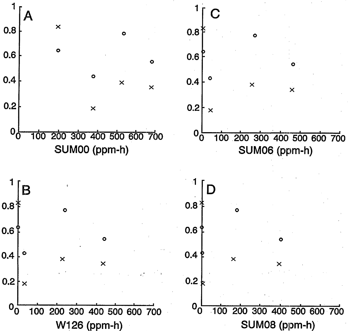
Figure 5-20. Reduction in volume production of loblolly pine seedlings (family 91) in relation to four exposure indices (A through D) (Lefohn et al., 1992a).
