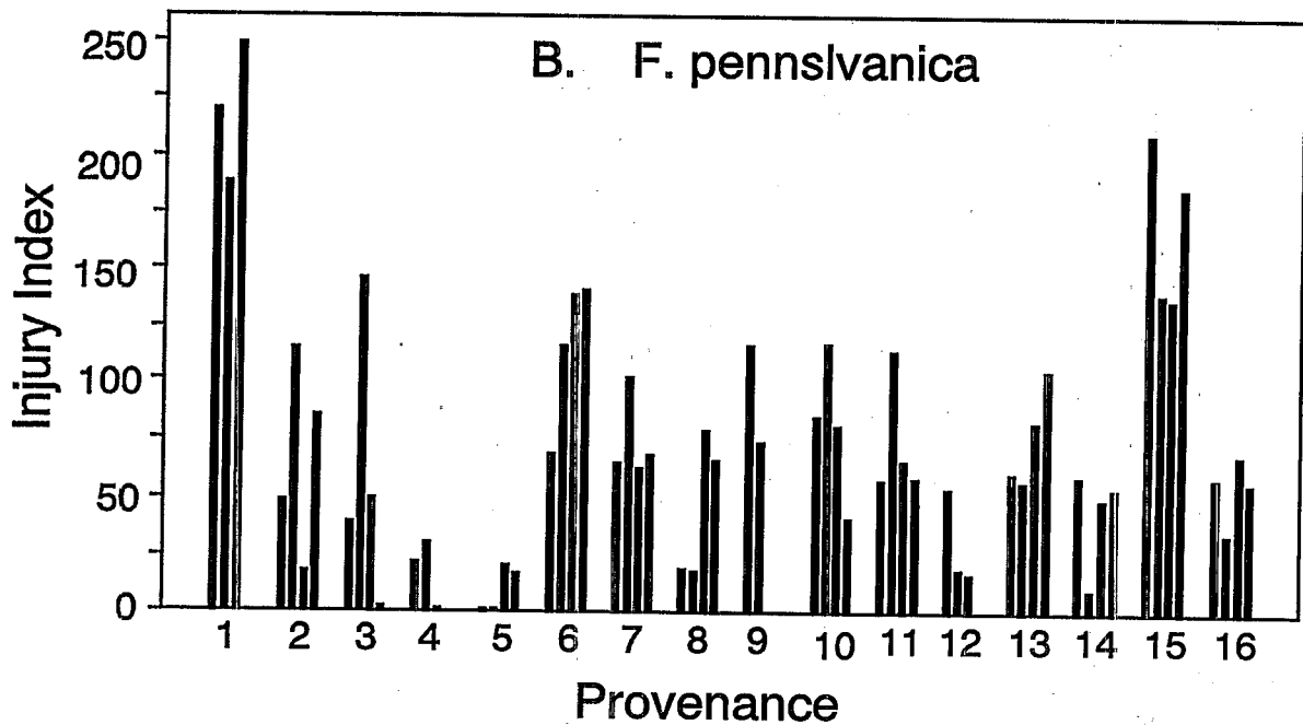
Figure 5-7. The average injury index for visible foliar injury after exposure of 1-year-old seedlings to 50 pphm ozone for 7.5 h. Each mean shown represents the average of five trees per family. There were either four or five half-sib families for each white ash ( Fraxinus americana L.) provenance (geographic location) and either three or four families for each green ash ( F. pennsylvanica Marsh.) provenance. The specifics of the experimental design are reported in Karnosky and Steiner (1981).
