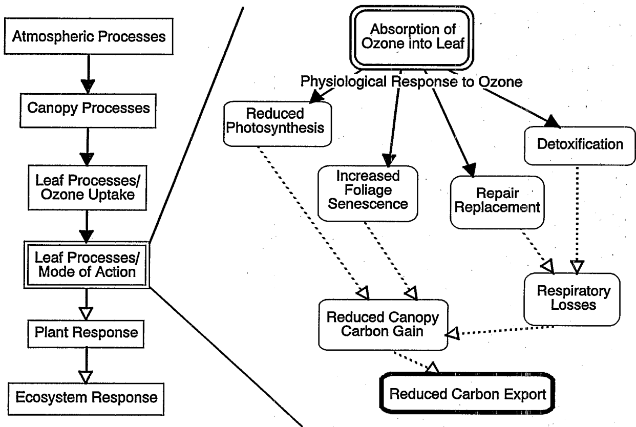
Figure 5-5. Effects of ozone ( O_3 ) absorption into a leaf. Once inside the leaf, O_3 can have a number of effects, all of which affect carbohydrate production and utilization. Reduced photosynthesis, increased leaf senescence, production of detoxification systems, and increased respiration (both maintenance and growth) reduce the amount of carbohydrate available for allocation. Compensation through production of new leaves, for instance, can counter some or all of these effects, depending on the O_3 exposure, the physiological state of the plant, and the species. Integration of these processes leads to changes in the amount of carbohydrate available for allocation from the canopy. Solid black arrows denote O_3 flow, and dotted arrows show the cascade of effects of O_3 absorption on leaf function. Boxes at the left and at the top with double borders indicate leaf processes; the box at the bottom with a dark border indicates the impact.
