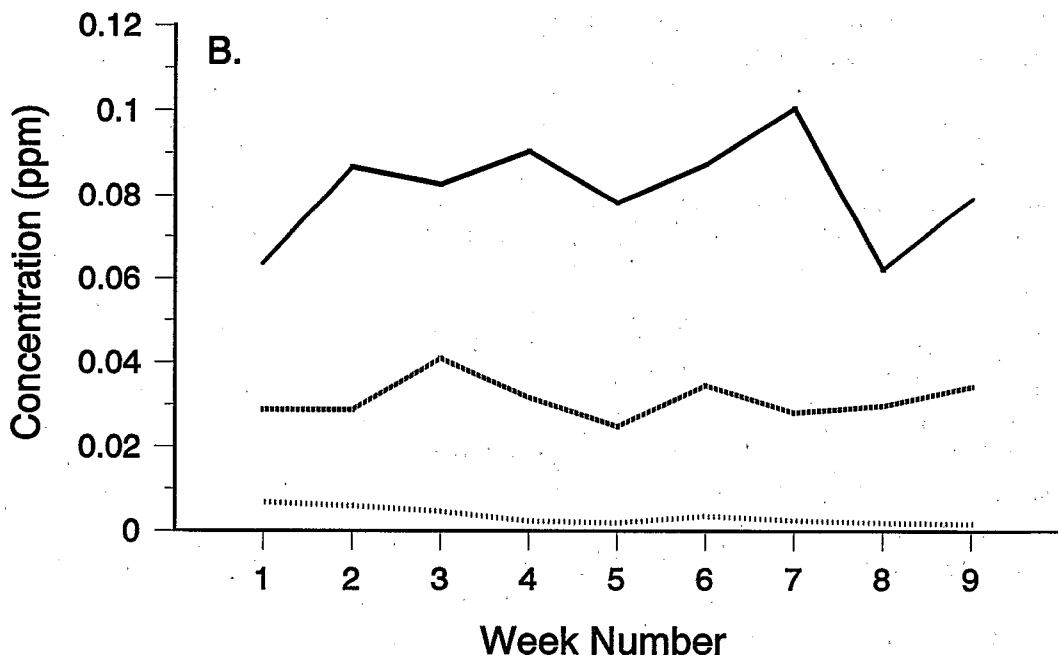
Figure 5-28. (A) Summary hourly ambient ozone ( O_3 ) concentrations during 9 weeks of experimentation (1990) at Montague-Amherst, MA, and (B) summary hourly ambient O_3 concentrations during 9 weeks of experimentation (1990) at Mount Equinox.
