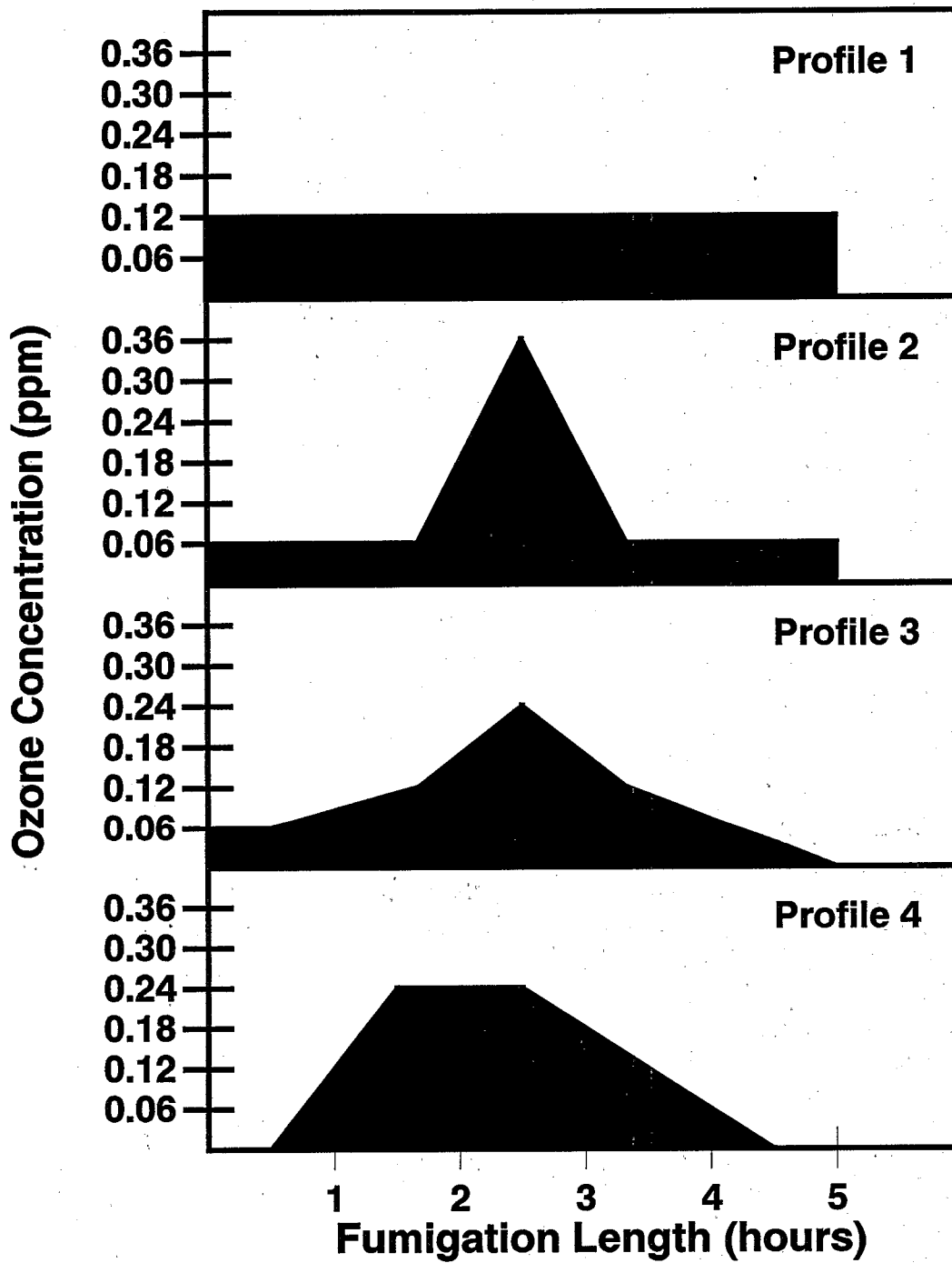
Figure 5-24. Experimental ozone exposure profiles.
