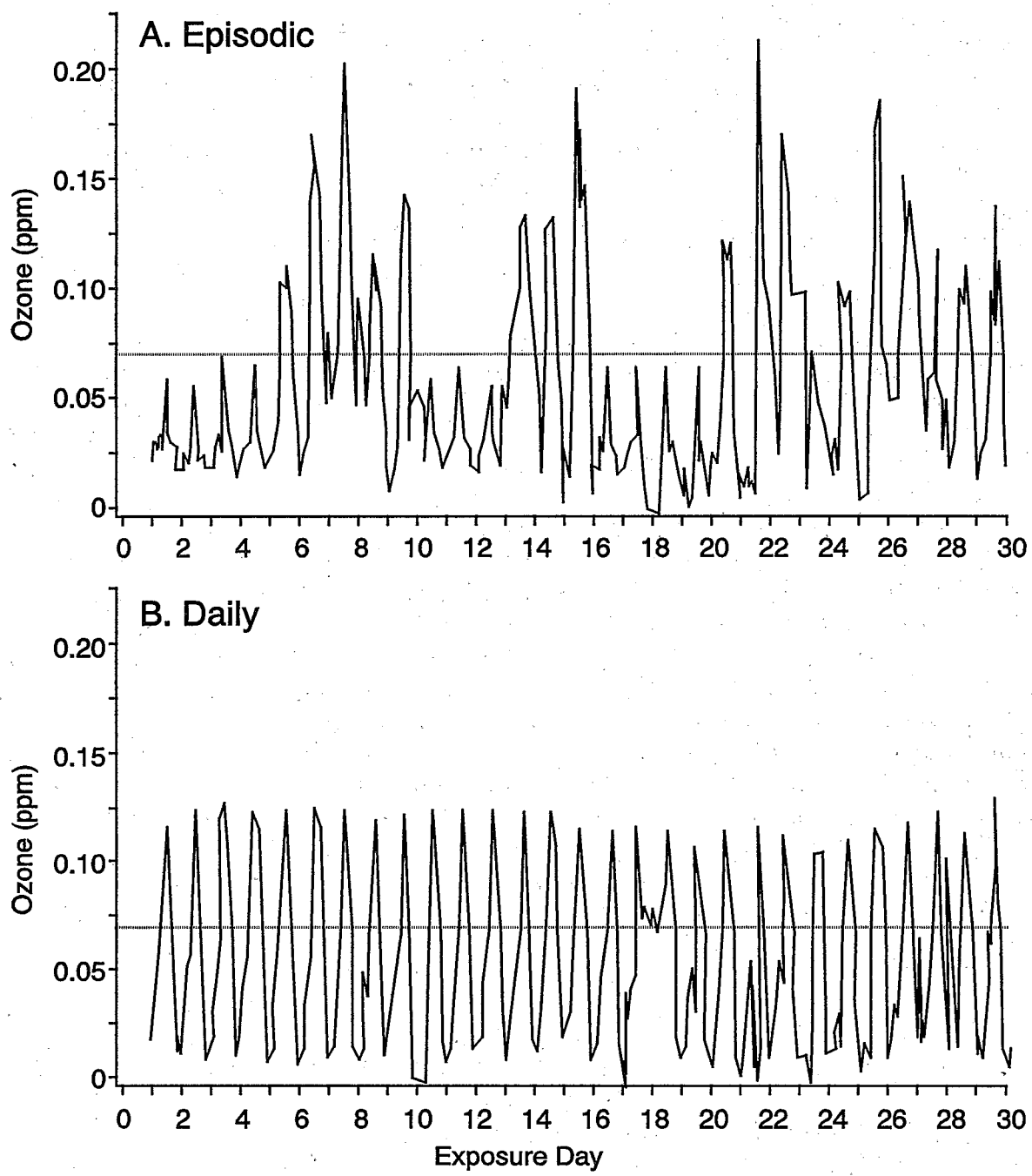
Figure 5-25. Ozone exposure profiles for the 1983 season.
