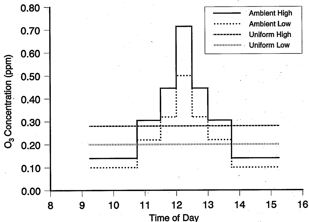
Figure 5-22. Fumigation schedule of uniform and simulated ambient ozone ( O_3 ) concentration distributions at two equivalent dose levels.
