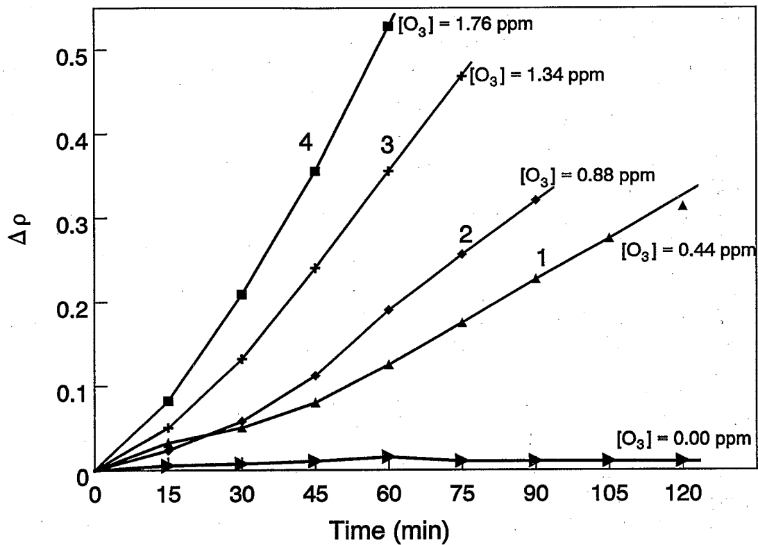
Figure 5-39. Relative decrease in stress ( \Delta\rho ) with time as a function of ozone concentration for polyisoprene vulcanizate.
