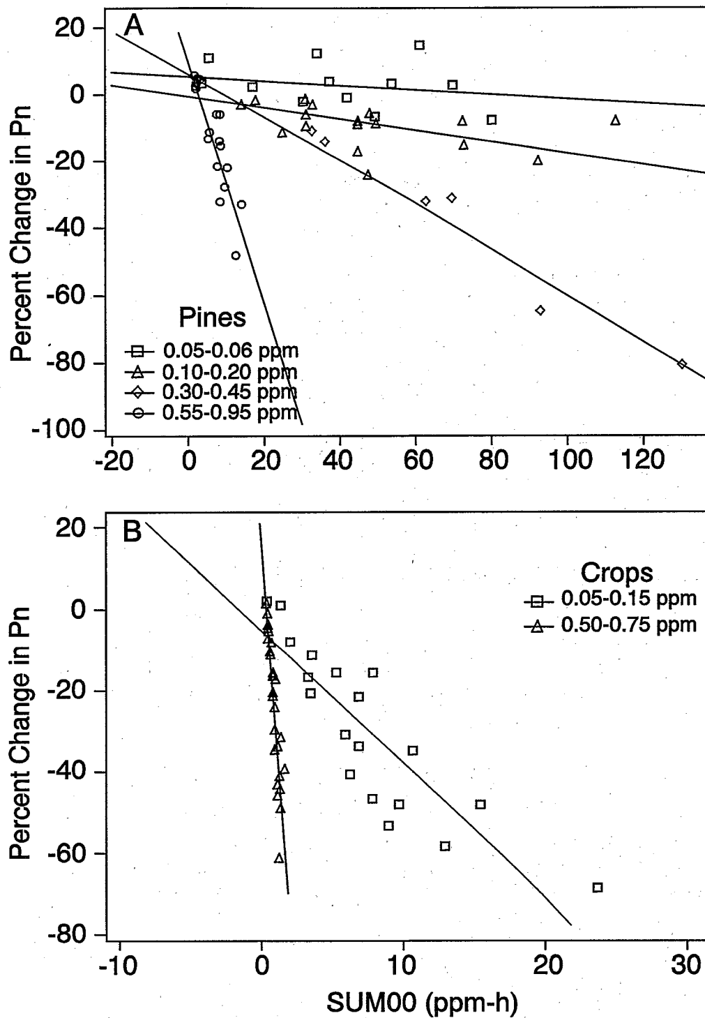
Figure 5-15. Percent reduction in net photosynthesis (Pn) of (A) pines (including one point for red spruce) and (B) agricultural crops in relation to total ozone exposure (SUM00), for several ranges of peak concentrations (Reich, 1987).
