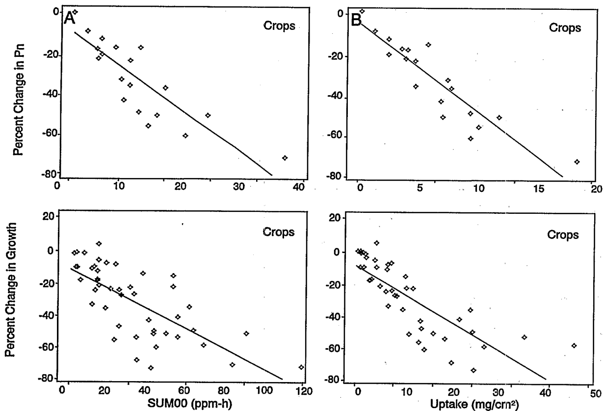
Figure 5-18. Percent reduction in net photosynthesis (Pn) and biomass growth of agricultural crops in relation to (A) total exposure (SUM00) and (B) estimated total ozone uptake (Reich, 1987).
