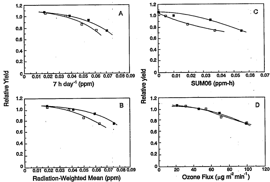
Figure 5-14. Quadratic exposure-response curves for the relative effect of ozone on grain yield of spring wheat in 1989 and 1990, using four different exposure indices (A through D).
