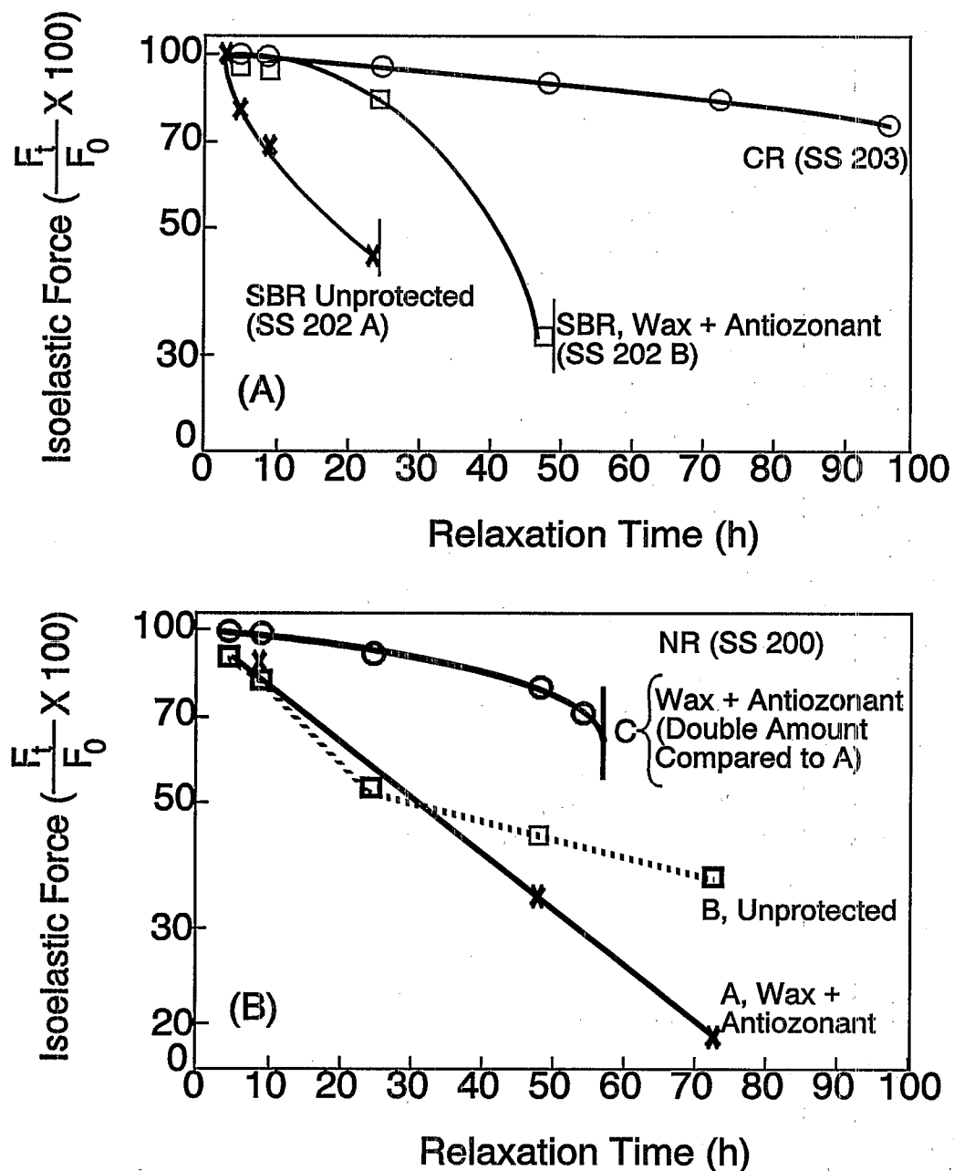
Figure 5-40. Relaxation of rubber compounds in ozone ( O_3 ) is affected by the combination of rubber formulation and type of O_3 protection. Compounds SS 202B (A) and SS 200C (B) were tested at an O_3 concentration of 0.5 ppm, a temperature of 30 °C, and elongation of 50%. The vertical lines at the end of curves mean total failure, and vertical axes represents relaxation, where F_0 is the initial force, and F_t is the force after time t .
