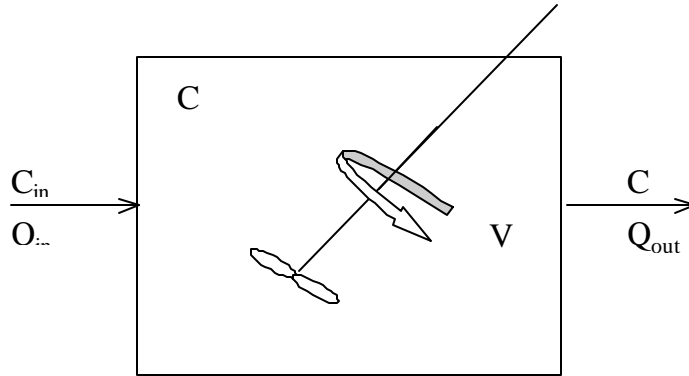
Figure 2-2. Continuous-flow stirred-tank reactor.
