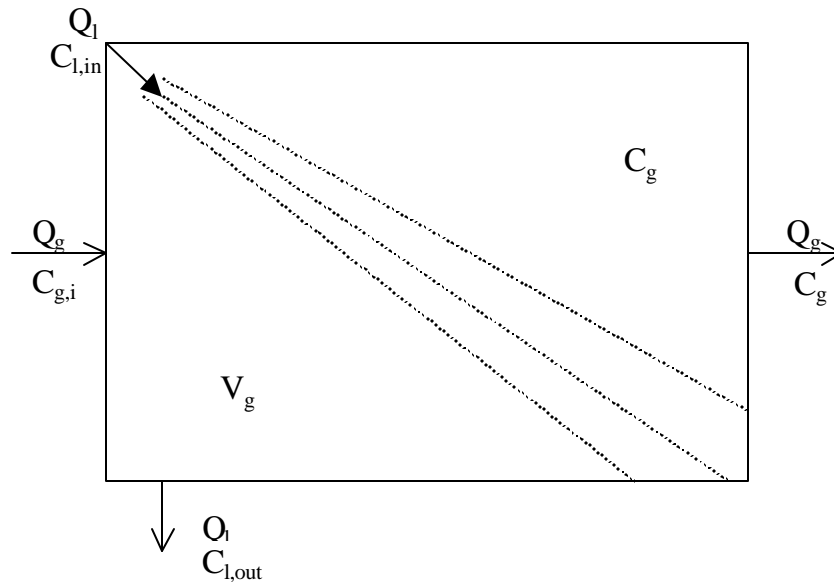
Figure 2-7. Shower model.
