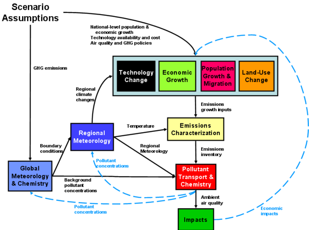
Figure F-2. Conceptual framework outlining the influence of global change factors on air quality. Black arrows represent linkages. Blue dashed arrows represent feedbacks.
