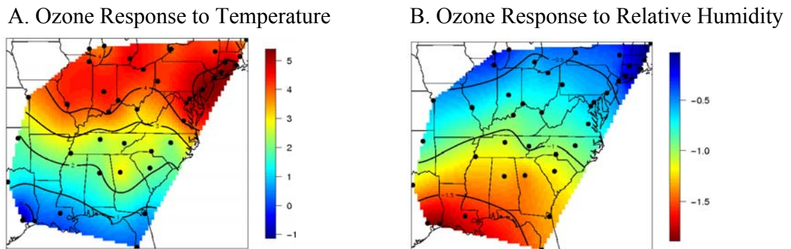
Figure A-2. Trends in ambient O 3 concentration sensitivities with respect to temperature and humidity. Red corresponds to areas with the greatest sensitivity to the parameter. Blue corresponds to areas showing the lowest sensitivity to the parameter. Panel A. Percent change in ozone per 1 degree (°C) increase in maximum 1-hour temperature. Panel B. Percent change in ozone per 1% increase in mid-day relative humidity.
