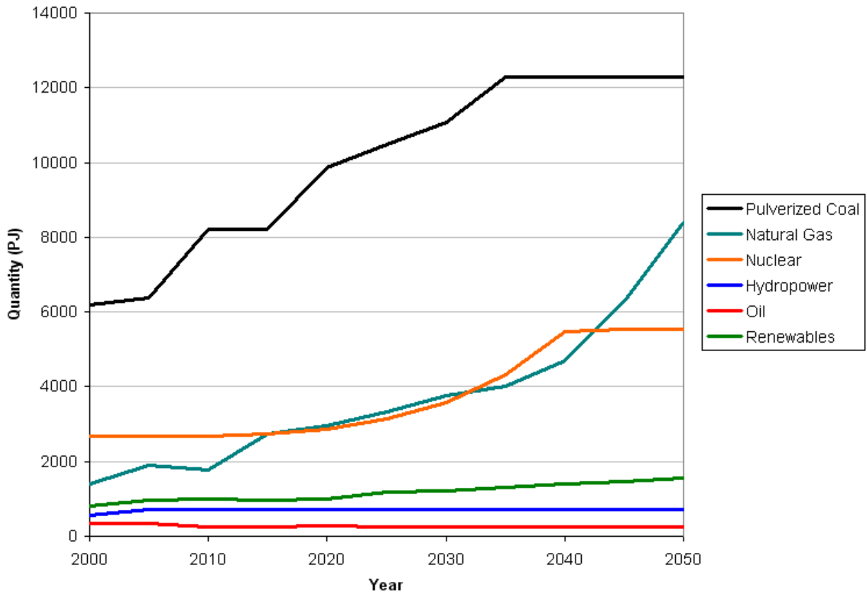
Figure F-7. Electricity generation by type of fuel. A breakdown of the renewables category is provided in Figure G-8.
