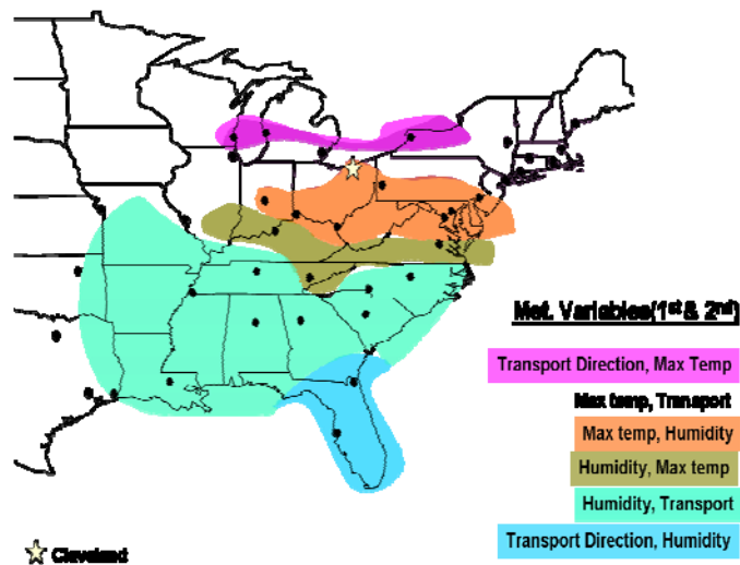
Figure A-1. Patterns of O 3 sensitivity to wind direction, temperature, and humidity, in the eastern portion of the United States.
