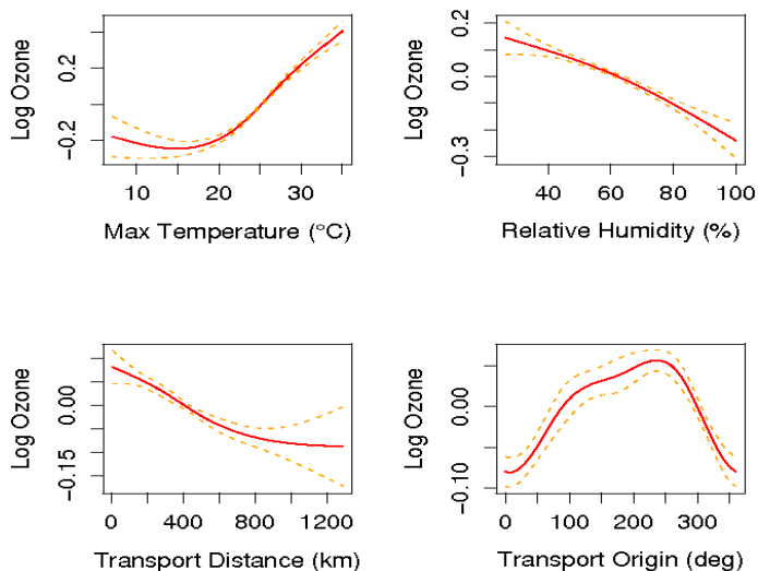
Figure A-3. Ozone response to changes in the four important meteorological parameters affecting ozone for Cleveland, OH. (Vertical axis units: log of the observed \text{O}_3 concentrations after correction for overall average, e.g. accounting for the other variables considered in the regression analysis.) Panel A: the \text{O}_3 response to temperature is relatively small for temperatures below \sim 20^\circ\text{C} but is strongly positive above 20^\circ\text{C} . Panel B: Decreasing \text{O}_3 with increasing relative humidity reflects increased cloudiness and atmospheric instability. Panel C: \text{O}_3 concentrations are inversely proportional to transport distance, e.g., the distance traveled by the incoming air mass over the previous 24-hours, reflecting the dilution effect of higher wind speed. Panel D: For Cleveland, the largest increment in ozone occurs when transport winds are from a southwesterly direction (i.e., 200 to 250 deg).
