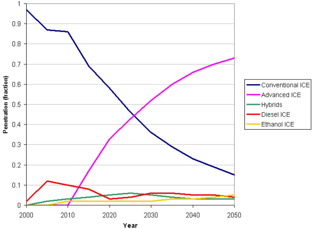
Figure F-9. Technology penetration into the light duty vehicle fleet.
