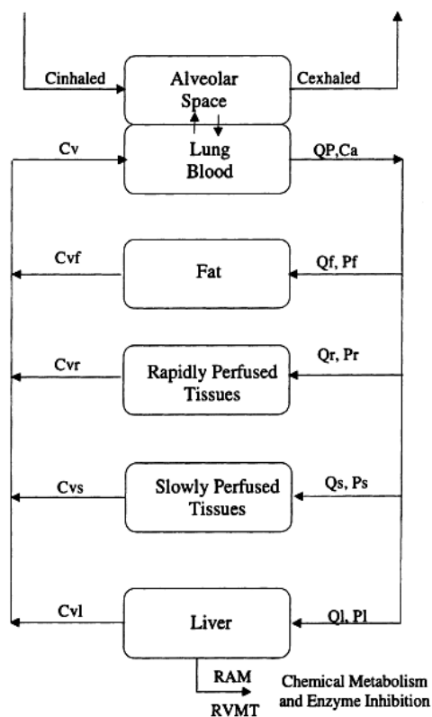
Figure 3-2. PBTK model for cis- and trans-1,2-dichloroethylene in rats.
