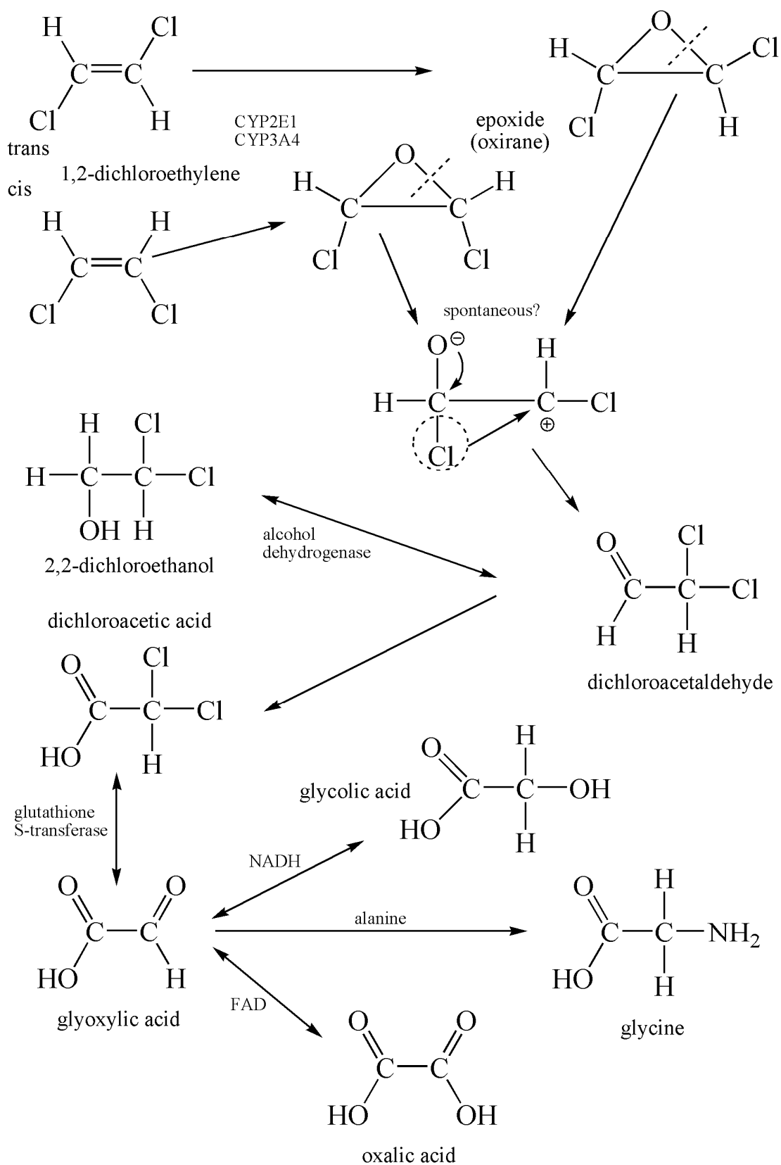
Figure 3-1. Proposed Metabolic scheme for cis- and trans-1,2-dichloroethylene.
