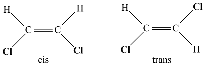
Figure 2-1. Chemical structures of cis- and trans-1,2-dichloroethylene.
