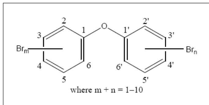
Figure 2-1. General structure of polybrominated diphenyl ethers.
