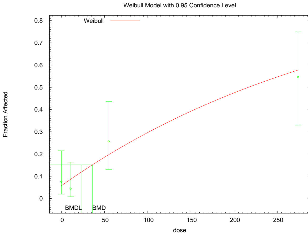
Figure C-5. BMD Weibull model of liver hyperplasia incidence data for F344 male rats exposed to 1,4-dioxane in drinking water for 2 years to support the results in Table C-4.
