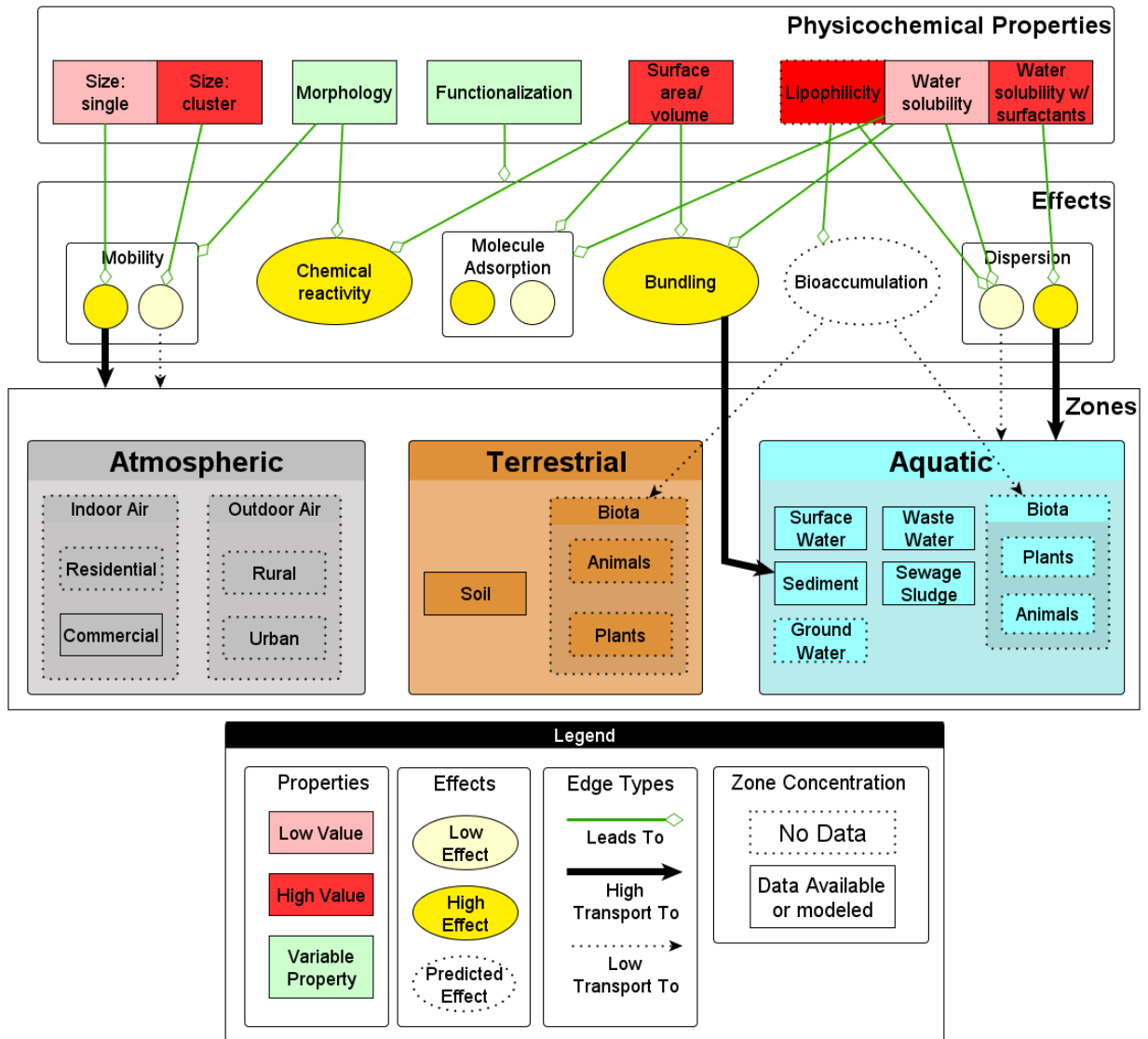
Figure J-2. Physicochemical properties map for multiwalled carbon nanotubes.
