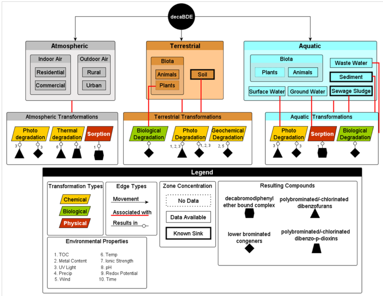
Figure J-5. Transformation map for decabromodiphenyl ether.
