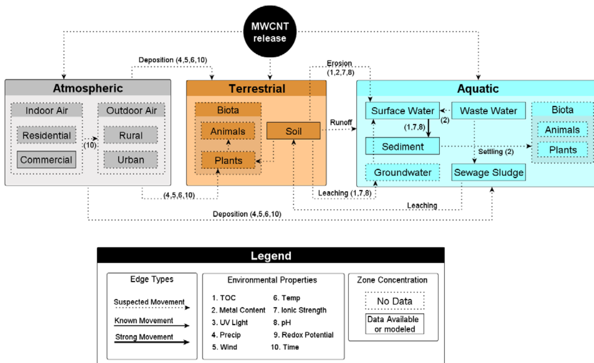
Figure J-4. Transport map for multiwalled carbon nanotubes.
