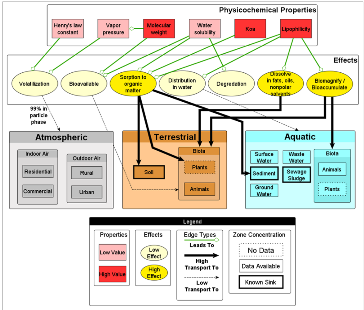
Figure J-1. Physicochemical properties map for decabromodiphenyl ether.
