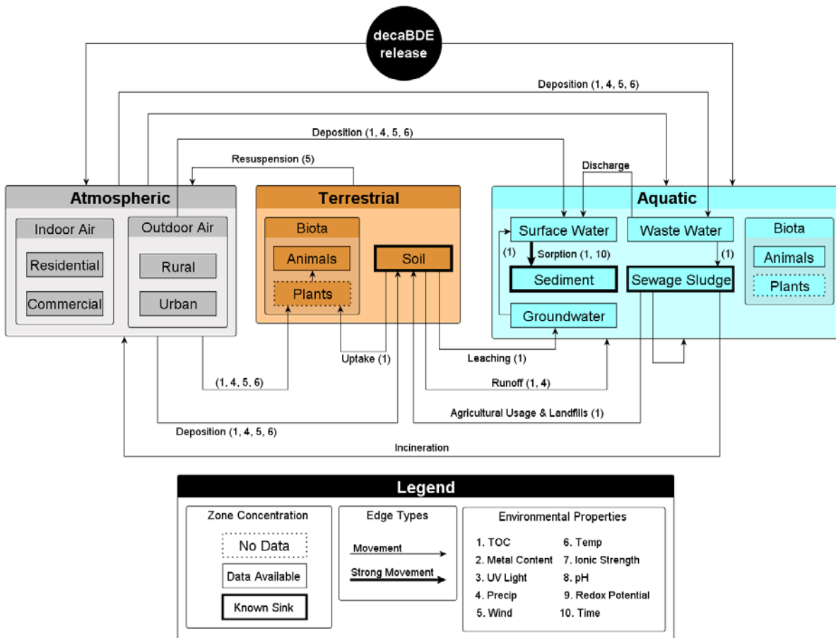
Figure J-3. Transport map for decabromodiphenyl ether.
