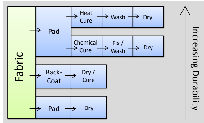
Figure 1-4. Durability of additive flame retardants.
