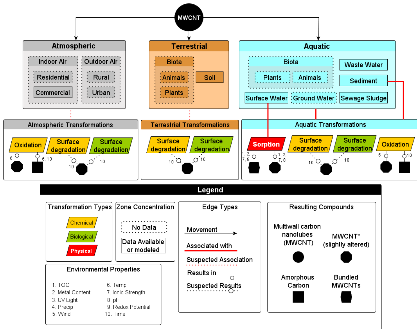
Figure J-6. Transformation map for multiwalled carbon nanotubes.
