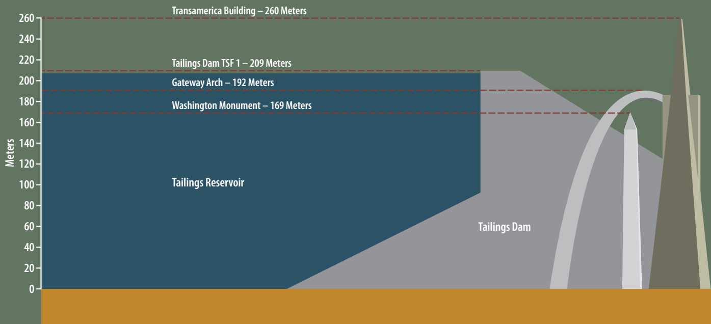
Height of the Dam at TSF 1 in the Pebble 2.0 and Pebble 6.5 Scenarios, Relative to U.S. Landmarks
